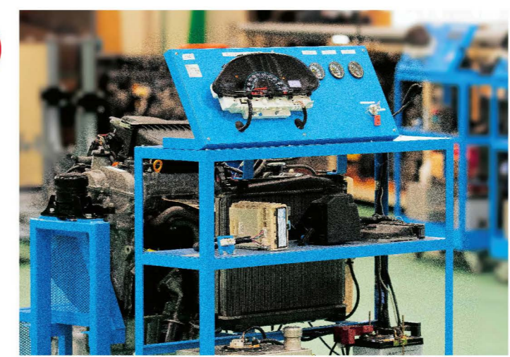
Engine bench
