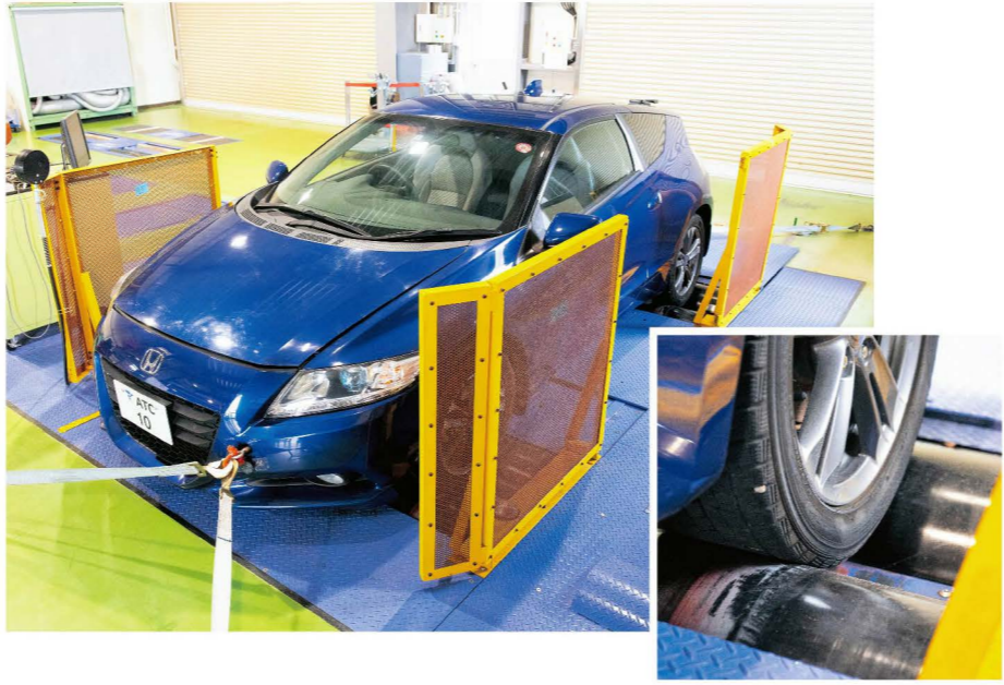
Chassis dynamometer
