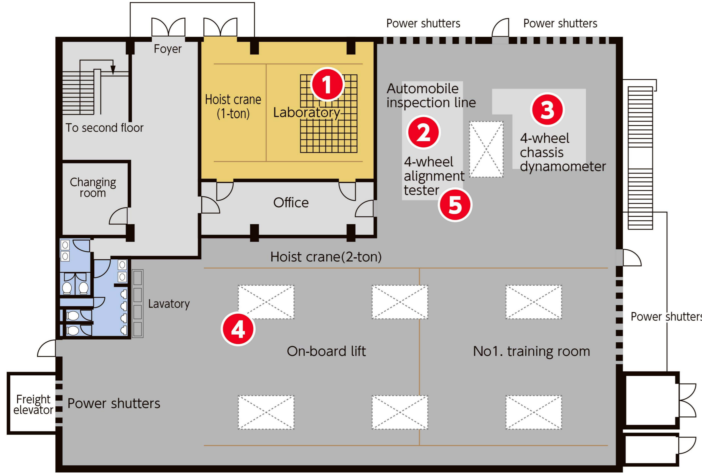
Alignment tester
