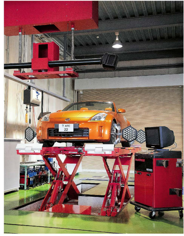
Alignment tester
